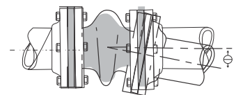
ANGULAR bending of the centerline
