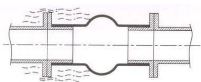
VIBRATION ISOLATION
