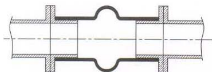
AXIAL CONTRACTION
