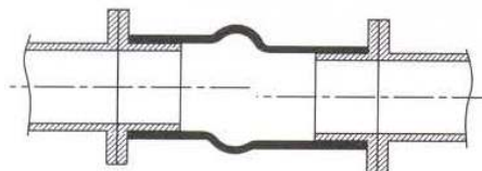
LATERAL DEFLECTION
